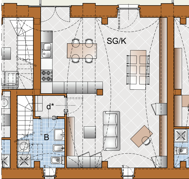
PIANO TERRA
