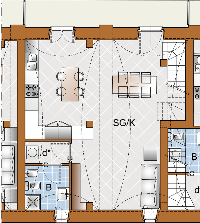
PIANO TERRA
